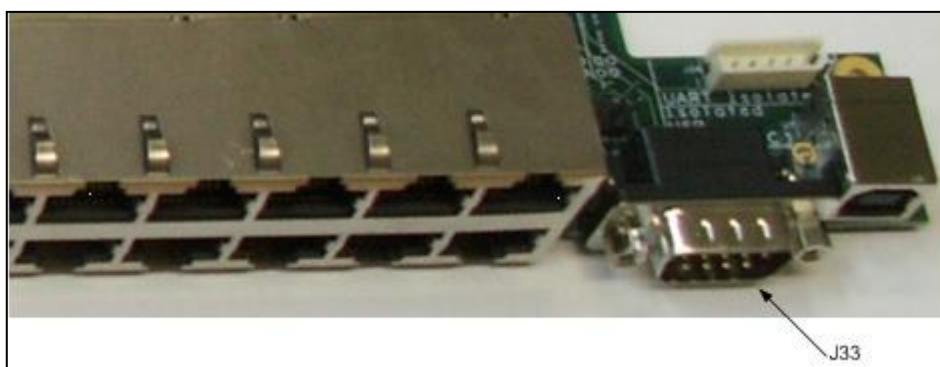
Figure 14: Isolated RS232
