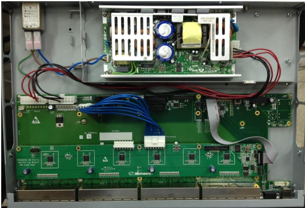
Figure 5: System in the Enclosure
