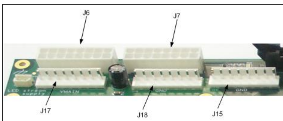
Figure 10: Vin Connectors
